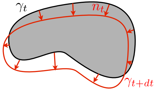
Fig. 3.1 Curve evolution in the normal direction.
