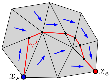
Fig. 2.10 Piecewise linear geodesic path on a triangulation.
