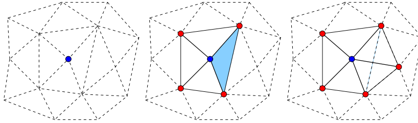
Fig. 2.8 Obtuse angle splitting : assume that the blue point x_i on the left image is to be updated. As shown on the middle image, its natural neighborhood B_\epsilon(x_i) with respect to the triangulation which represents the surface contains an obtuse angle. In order to perform the update, a farther point y needs to be added to B_\epsilon(x_i) such that B_\epsilon(x_i) \cup \{y\} does not contain an obtuse angle anymore.
