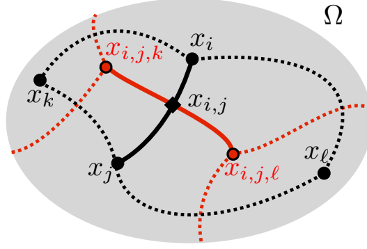
Fig. 4.1 Schematic diagram of Geodesic and Delaunay.
