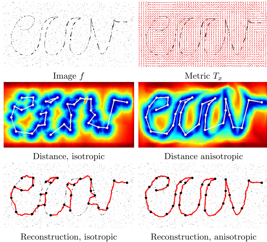
Fig. 4.24 Perceptual grouping using isotropic metric (left) and anisotropic metric (right).
