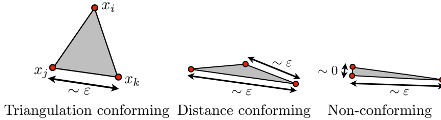
Fig. 4.4 Shapes of triangles with distance and/or triangulation conforming to the Euclidean constant metric.
