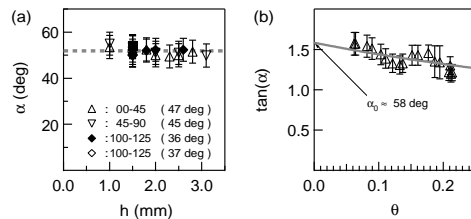
FIG. 3. (a) Angle \alpha vs. thickness h for \theta \simeq 0.21 – The angle \alpha neither depends on the thickness h of the granular layer nor on the grain size d and cohesion [Symbol : d ( \theta_a )]. (b) Angle \alpha vs. elongation \theta – The stretching induces a rotation of the stripes such that \tan(\alpha) = (2 - \theta)/[2(1 + \theta)] \tan(\alpha_0) . From the extrapolation of the data (grey line), one assesses the angle \alpha_0 \simeq 58 deg ( d=0-45 \mu\text{m} , h = 2 mm and \theta_a = 47 deg).
