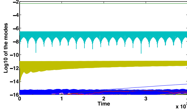
FIGURE 2. Evolution of the Fourier modes of the nonresonant solution in logarithmic scale: u_0(x) = 2 \cos(x_1) + 2 \cos(x_2)
