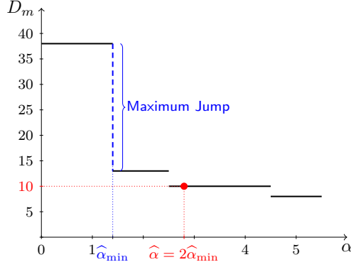
Figure 1: If \text{pen}_{\min} = \alpha_{\min} \cdot \text{pen}_{\text{shape}} , for a known penalty shape \text{pen}_{\text{shape}} , then one can estimate \alpha_{\min} by using the dimension jump. This gives \hat{\alpha}_{\min} and \text{pen}_{\text{opt}} = 2\hat{\alpha}_{\min} \cdot \text{pen}_{\text{shape}} is then an optimal penalty according to the slope heuristics.
