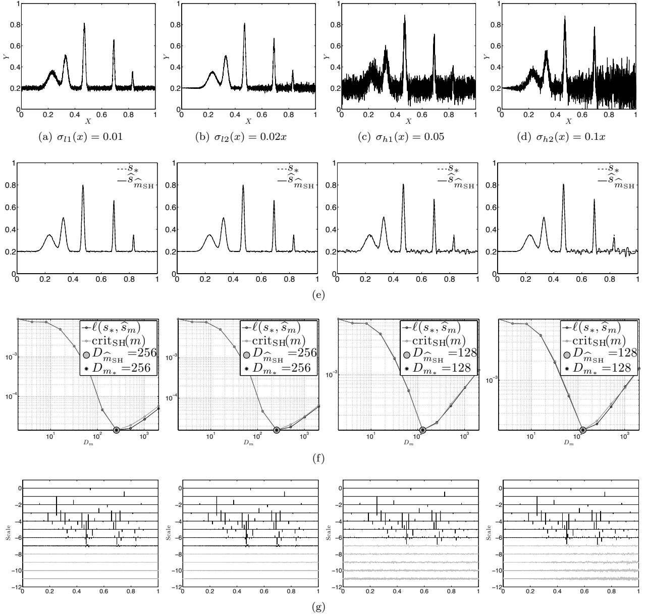
Figure 5: (a)-(d): Noisy version of Spikes for each \sigma(\cdot) scenarios. (e): Typical reconstructions from a single simulation with n = 4096 . The dotted line is the true signal and the solid one depicts the estimates \widehat{s}_{\widehat{m}_{SH}} . (f): Graph of the excess risk \ell(s_*, \widehat{s}_m) against the dimension D_m and (shifted) \text{crit}_{SH}(m) (in a log-log scale). The gray circle represents the global minimizer \widehat{m}_{SH} of \text{crit}_{SH}(m) and the black star the oracle model m_* . (g): Noisy and selected (black) wavelet coefficients (see Figure 3(e) for a visual comparison with the original wavelet coefficients).
