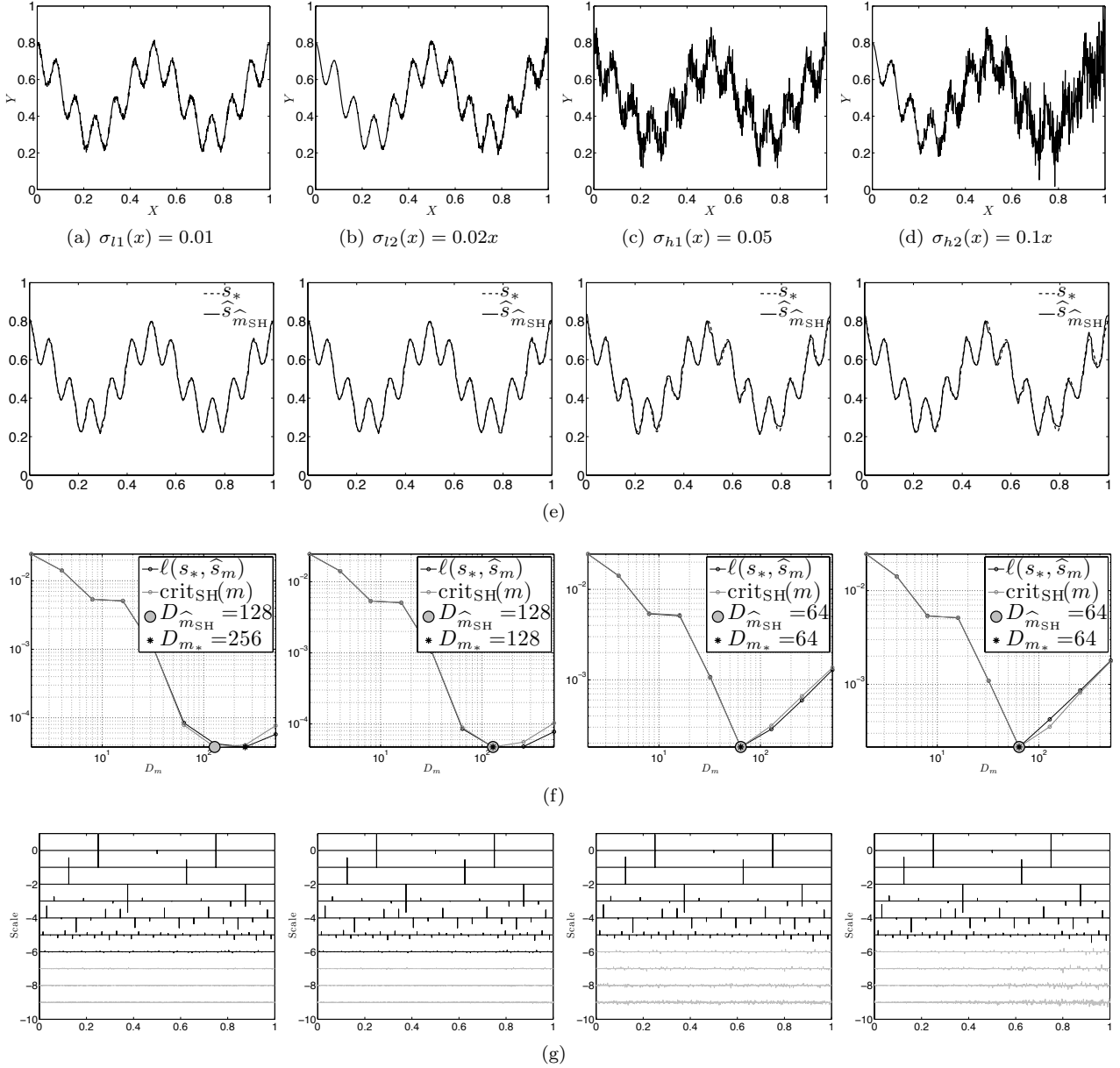
Figure 4: (a)-(d): Noisy version of Wave for each \sigma(\cdot) scenarios. (e): Typical reconstructions from a single simulation with n = 1024 . The dotted line is the true signal and the solid one depicts the estimates \hat{s}_{\widehat{m}_{SH}} . (f): Graph of the excess risk \ell(s_*, \hat{s}_m) against the dimension D_m and (shifted) \text{crit}_{SH}(m) (in a log-log scale). The gray circle represents the global minimizer \widehat{m} of \text{crit}_{SH}(m) and the black star the oracle model m_* . (g): Noisy and selected (black) wavelet coefficients (see Figure 3(e) for a visual comparison with the original wavelet coefficients).
