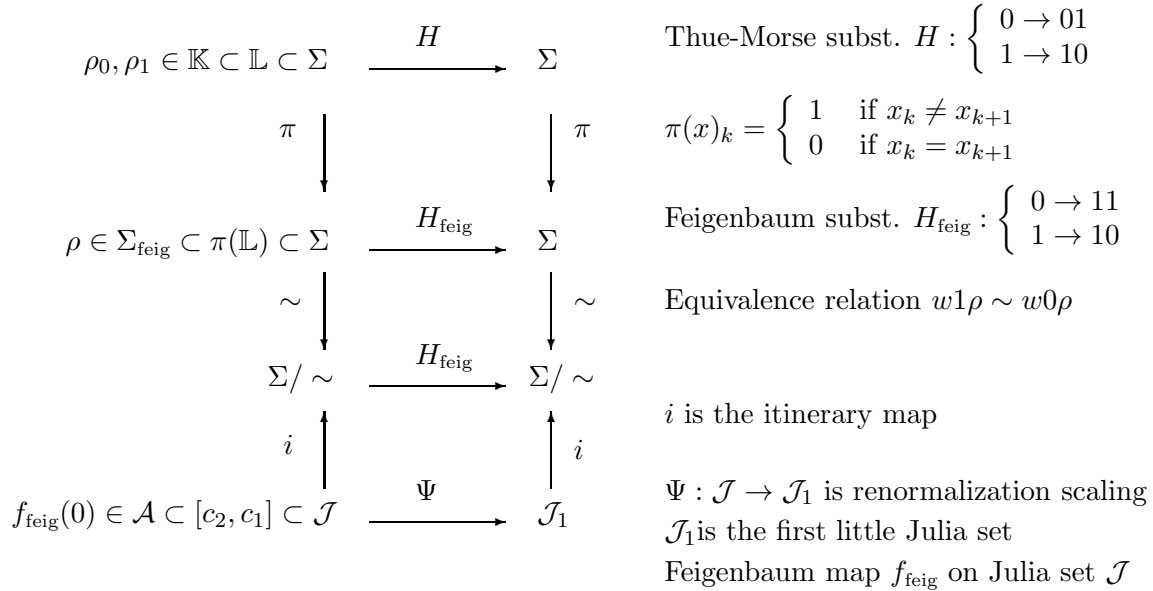
FIGURE 11. Commutative diagram linking the Thue-Morse substitution shift to the Feigenbaum map. Further commutative relations:
