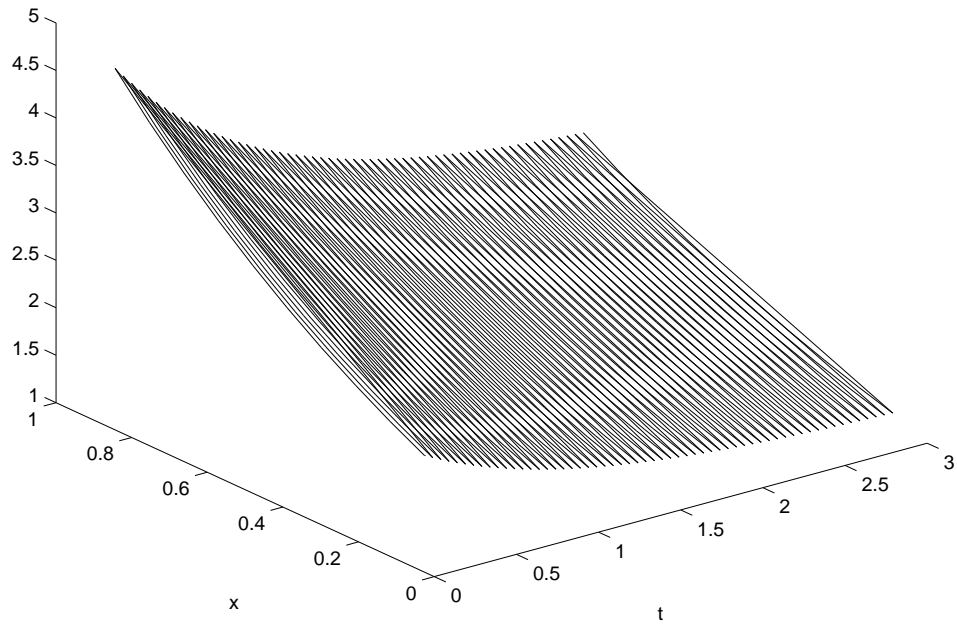
Figure 2. Exact solution
