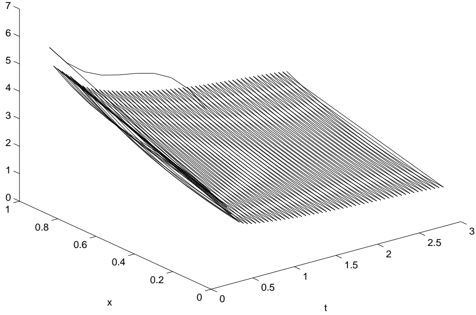
Figure 1. Approximated solution
