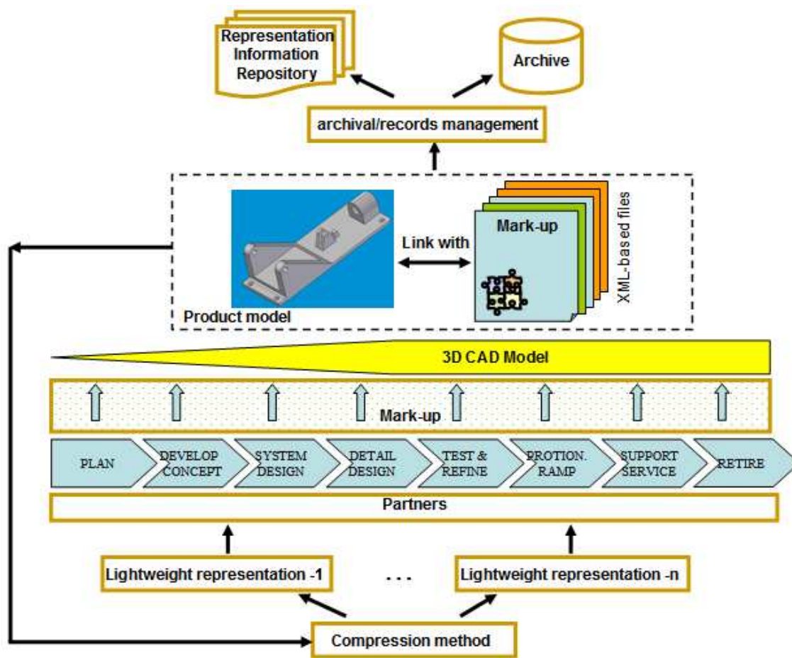
Figure 1 – Framework of lightweight representations in product lifecycle
