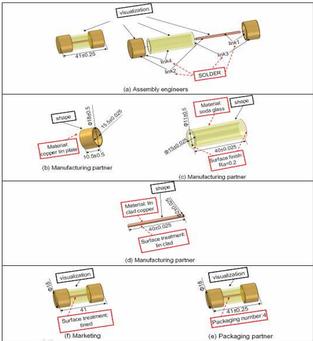
Figure 7 Markups for the fuse product
