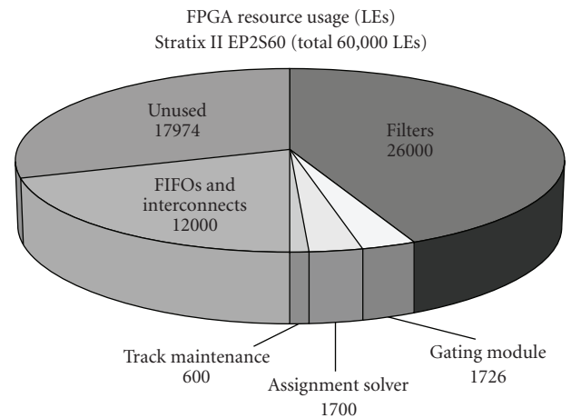
FIGURE 22: System Hardware Size.
