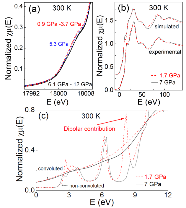
FIG. 5. (color online) (a) High-pressure Zr K edge XANES spectra obtained at 300 K. Note the pressure evolution of the PEFS. (b) Experimental and simulated XANES spectra at 1.7 GPa and 7 GPa. In b), the origin (0) corresponds to the Zr K edge. (c) The non-convoluted and convoluted theoretical PEFS at 1.7 GPa and 7 GPa showing the disappearance of the dipolar contribution at high pressure.
