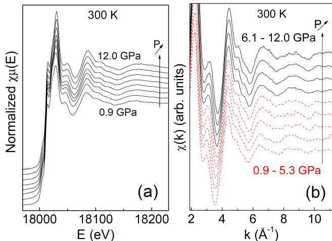
FIG. 2. (color online) (a) Normalized XAS spectra obtained at 300 K between 0.9 GPa and 12 GPa, (b) Extracted \chi(k) . Both signals are vertically shifted for clarity.
