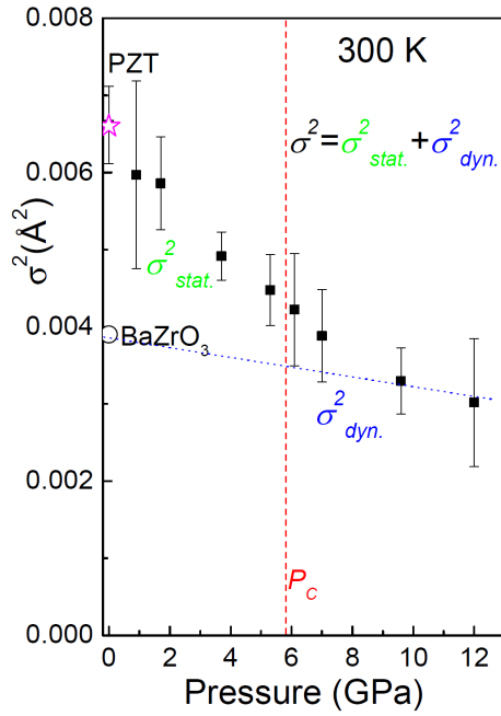
FIG. 4. (color online) Pressure behavior of the DWF for the Zr-O atom pairs at 300 K. Values reported in the literature for PZT 14 (*) and BaZrO 3 24 (o) are also included. P_C (the dashed line) corresponds to the paraelectric transition 9 . The dotted line represents the decrease of \sigma_{dyn.}^2 , as explained in the text.
