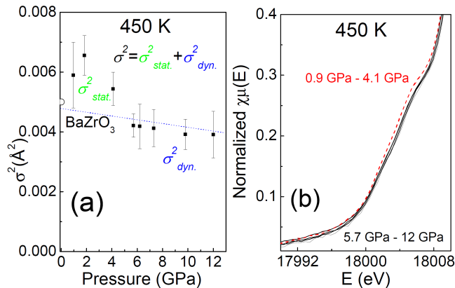
FIG. 6. (color online) (a) Pressure behavior of the DWF for the Zr-O atom pairs at 450 K. The calculated value for BaZrO 3 (○) 24 is also included. \sigma_{dyn}^2 (the dotted line) corresponds to a decrease of about 1% per GPa. (b) High-pressure Zr K edge XANES spectra obtained at 450 K. Note the pressure evolution of the PEFS.
