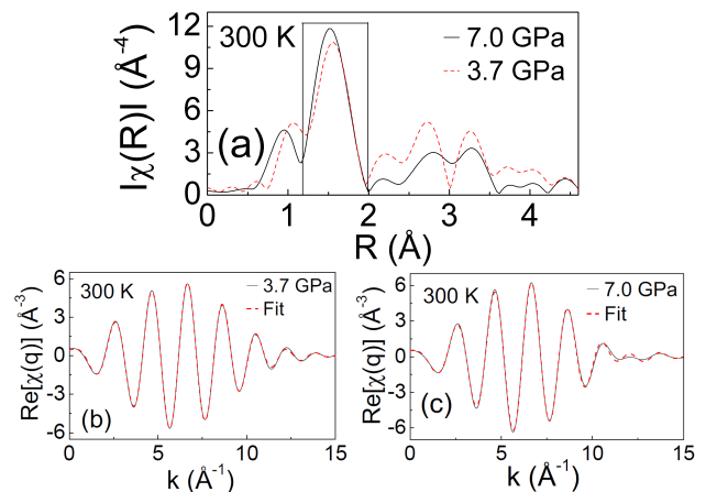
FIG. 3. (color online) (a) The k^3 -weighted EXAFS signals (obtained in the 2-11 \text{\AA}^{-1} range) are shown at 3.7 GPa (dashed) and 7.0 GPa (full). The Zr-O first coordination shell is extracted using a Hann window in the 1.2-2 \text{\AA} range. (b) and (c) The k^3 -weighted backward Fourier transforms along with the resulting fits (dashed) are shown at 3.7 GPa and 7 GPa, respectively.
