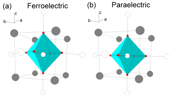
FIG. 1. (color online) (a) Ferroelectric state with a tetragonal ( P4mm ) crystal structure and (b) Paraelectric state with a cubic ( Pm\bar{3}m ) crystal structure. Pb atoms (grey) at each corner of the pseudocubic lattice with Ti/Zr (white) in the center. Oxygen atoms (red) are at the center of the faces. In the ferroelectric form below T_C or P_C , both Pb and Ti/Zr will have atomic displacements along [001] giving rise to the spontaneous polarization. The spontaneous polarization disappears in the paraelectric form above T_C or P_C .
