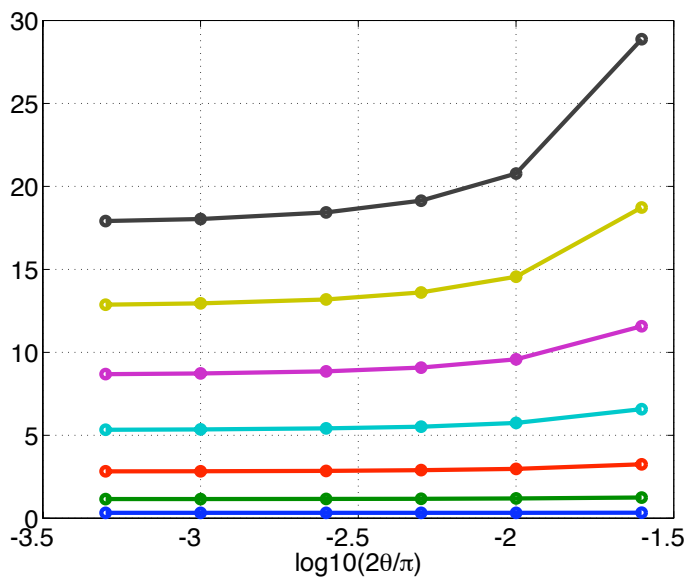
Figure 4: \rho_{n,2}(\theta) (ordinates) versus \log_{10}(2\theta/\pi) (abscissa). n = 1, \dots, 7 (bottom to top).
