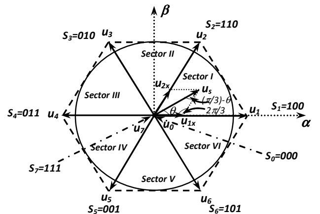
Fig. 4. Space vectors.
