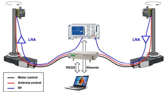
Fig. 3 Schematic diagram of the measurement equipment
