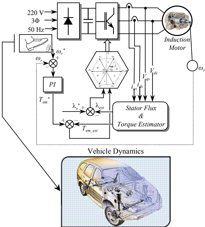
Fig. 2. DTC general configuration.
