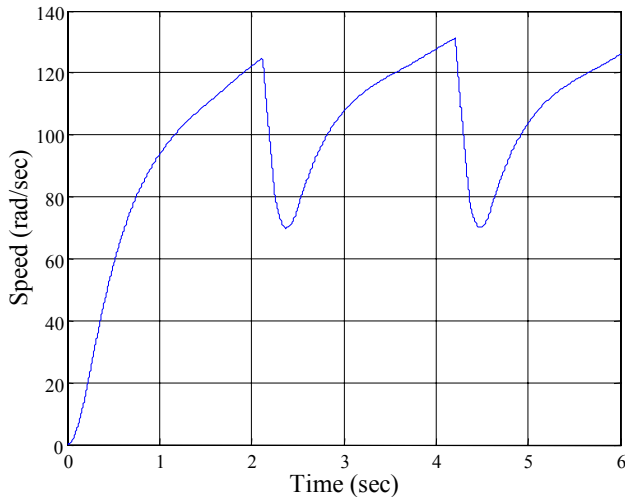
Fig. 6. Speed curve.
