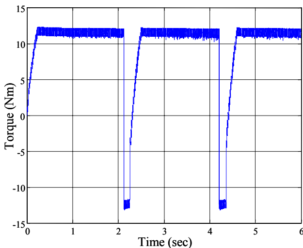
(b) Estimated torque.
