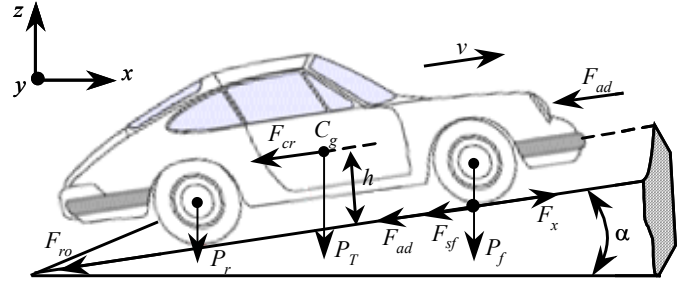
Fig. 1. Elementary forces acting on a vehicle.
