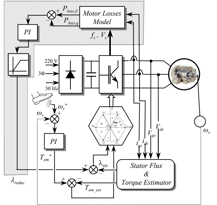
Fig. 3. Scheme for energy optimal model-based control.
