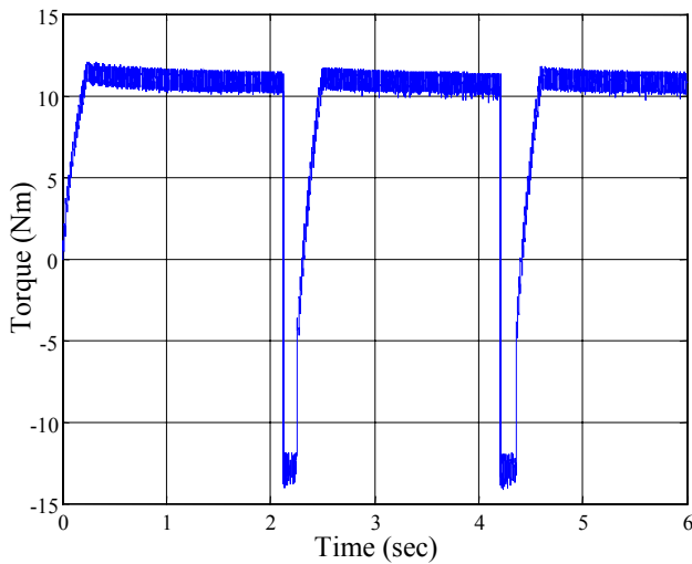
(a) Developed torque.
