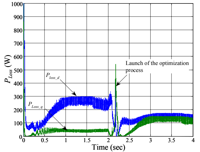
(b) P_{lossd} and P_{lossq} variations.
