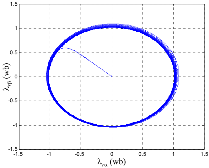
(a) Without optimization.
