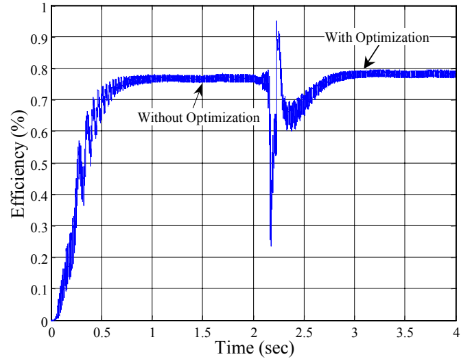
(a) Efficiency.
