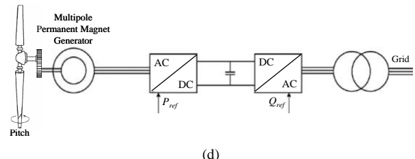
Fig. 9. Full-scale power electronics WECS: (a) Induction generator, (b) Synchronous generator, (c) Multipole synchronous generator, (d) Multipole permanent magnet generator.
