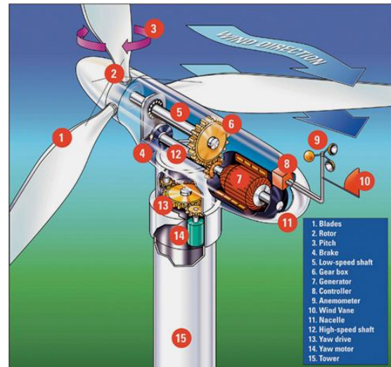
Fig. 3. Cutaway of a wind turbine nacelle.
