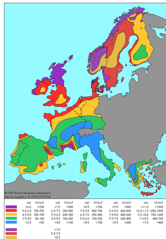
Fig. 1. Wind resources in Western Europe (according to RISOE, for the European Commission).
