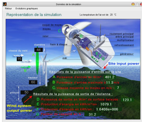
Fig. 14. Simulation window.
