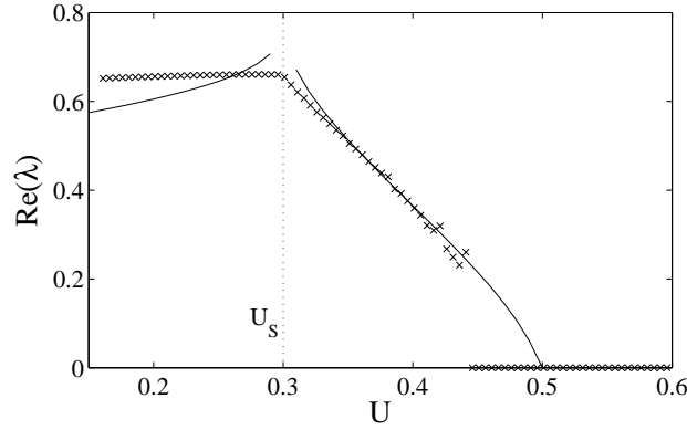
Figure 2. Growth rate \text{Re}(\lambda) (full line) of the instability of the inhomogeneous waterbag states obtained by solving Eq. (33) for waterbags with boundary energy U . The crosses are the results of numerical simulations of the N -body Hamiltonian. The agreement between theory (which describes the N \rightarrow \infty limit) and numerics (which is performed at N = 3 \times 10^5 ) is reasonably good apart from the region near the separatrix energy U_s = 0.3 and the one near the critical energy U_c = 0.498 , which is theoretically determined by solving Eq. (42).
