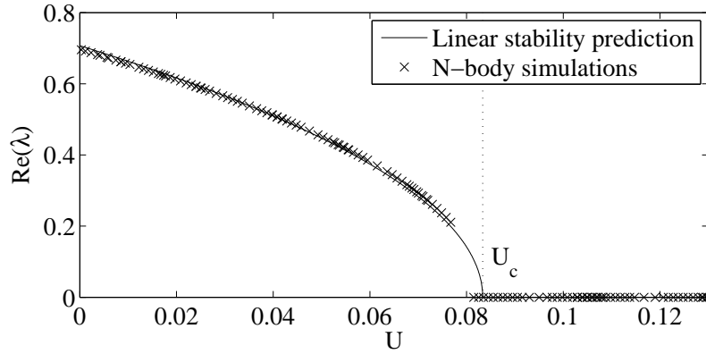
Figure 3. Growth rate \text{Re}(\lambda) of the instability (full line) as a function of the energy U for the HMF model (model (27) with \kappa = 0 ), as obtained analytically in formula (52). The crosses are the results of exponential fits of the short-time evolution of the magnetization for the N -body HMF Hamiltonian.
