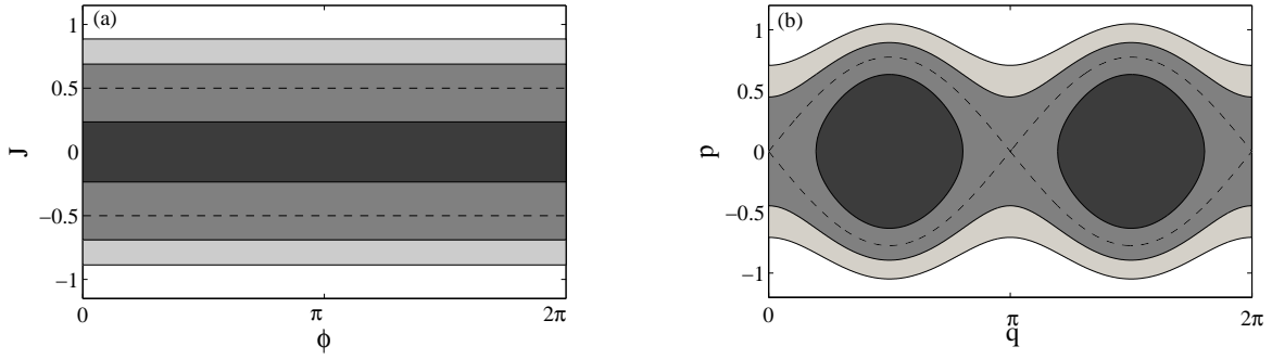
Figure 1. Waterbags in action-angle (panel a) and in (q, p) space (panel b). The waterbags have increasing boundary energies U = 0.2, 0.4 and 0.55 and they are represented by filled contours of lighter and lighter grey as the energy is increased. The dashed line corresponds to the separatrix, which has energy U_s = 0.3 and action J_s = 0.5 .
