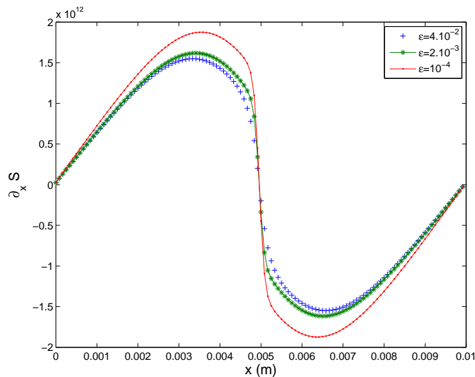
Figure 4: Gradient of the potential \partial_x S for different values for \epsilon at time t = 80 s.
