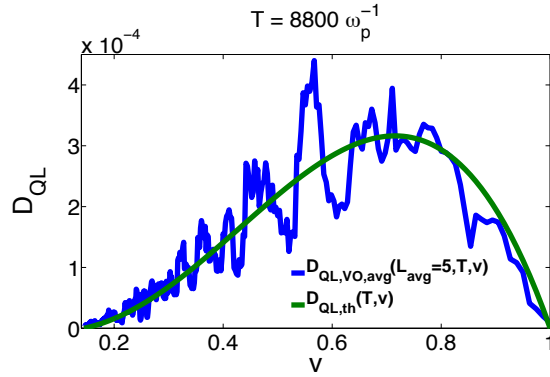
(b) D_{QL,avg}(T, v) vs. D_{QL,th}(T, v)
