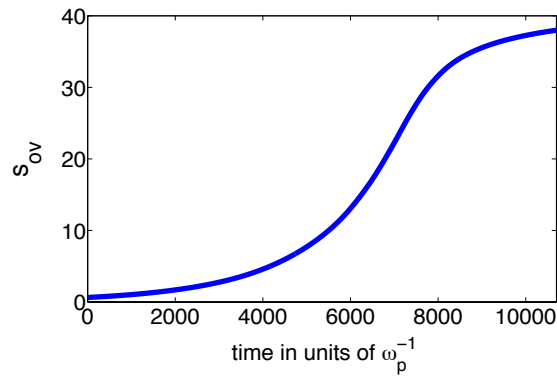
(c) s_{ov}
