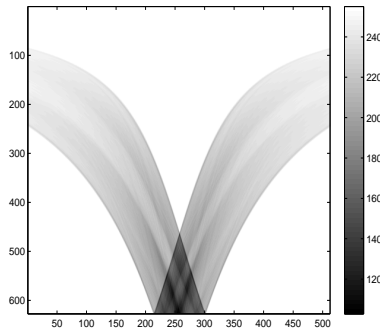
Fig. 6 The TV transform of the Shepp-Logan image shown in Fig. 5 with d\omega = 0.005 rad.
