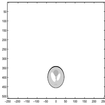
Fig. 5 Original Shepp-Logan phantom
