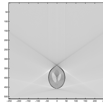
Fig. 8 FBP-IM reconstruction of the Shepp-Logan image with d\omega = 0.0025 rad, the quality is slightly improved compared to Figure 7.
