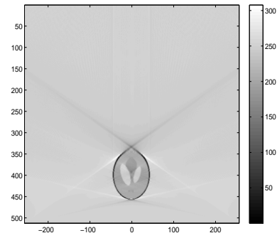
Fig. 7 FBP-IM reconstruction of the Shepp-Logan image with d\omega = 0.005 rad.
