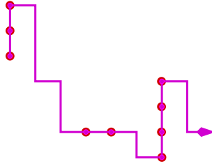
FIGURE 8. The factorization of a proper NES-walk.
