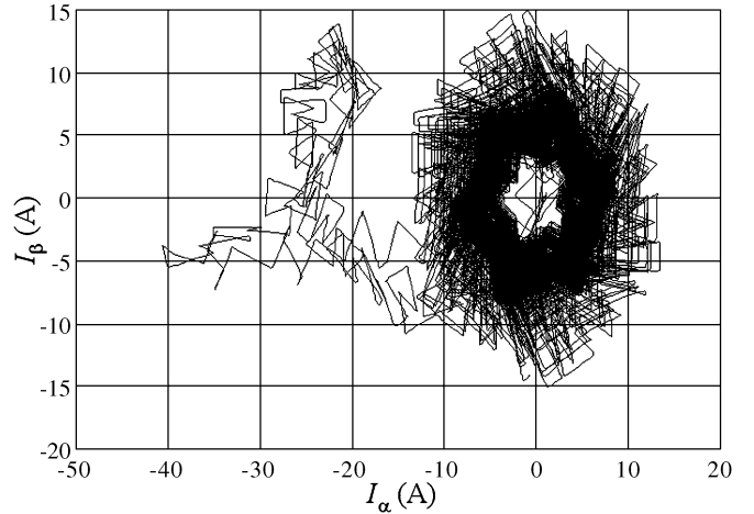
Fig. 2. Current pattern in case of T_1 misfiring.
