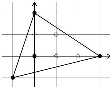
FIGURE 1. Newton polygon of F = x^{-1}y^{-1} + 1 + 2x^3 + 3y^2 .
