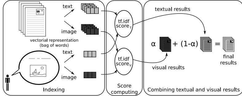
Fig. 1. Multi-modal IR model
