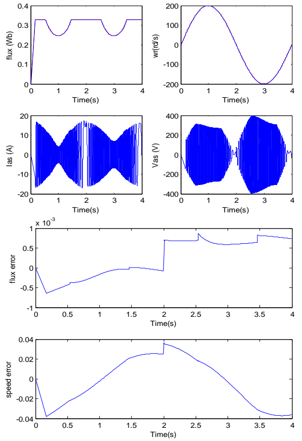
Fig. 5. PI/Backstepping: Test 3.
