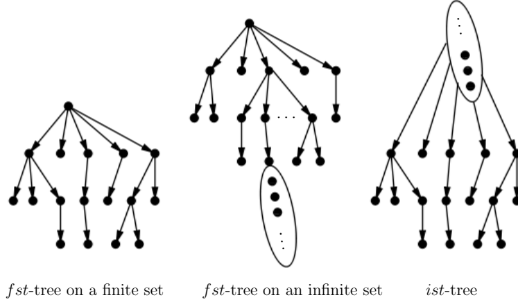
Figure 2: Underlying trees of source transitive trees
