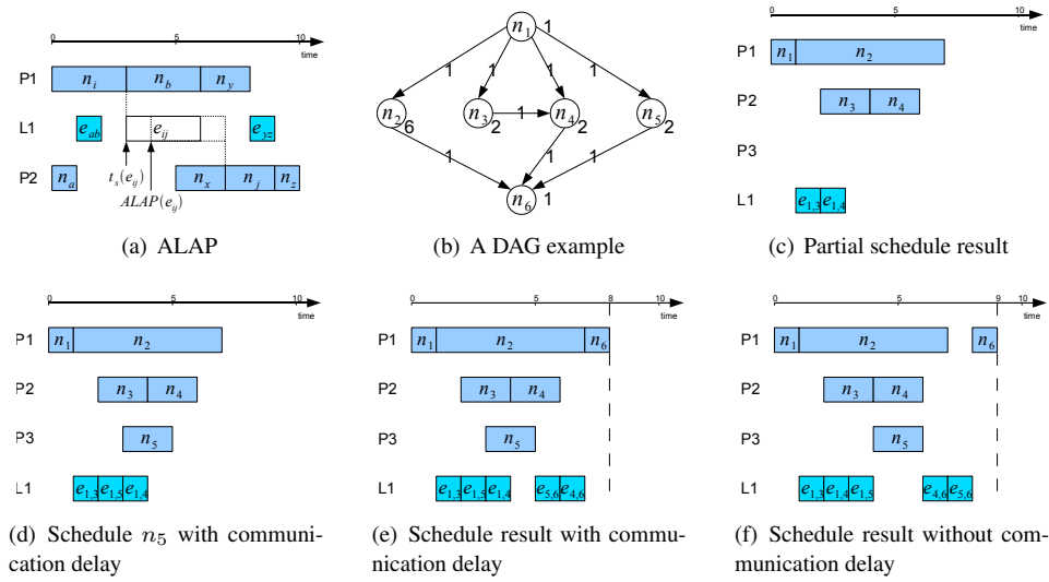
Figure 4: Communication delay
