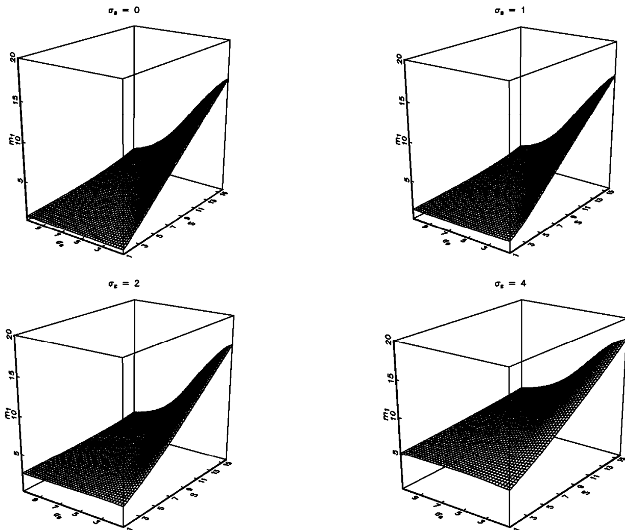
Figure A: The average size of price changes as a function of model parameters ( S , \sigma_S ) for different values of \sigma_\varepsilon
