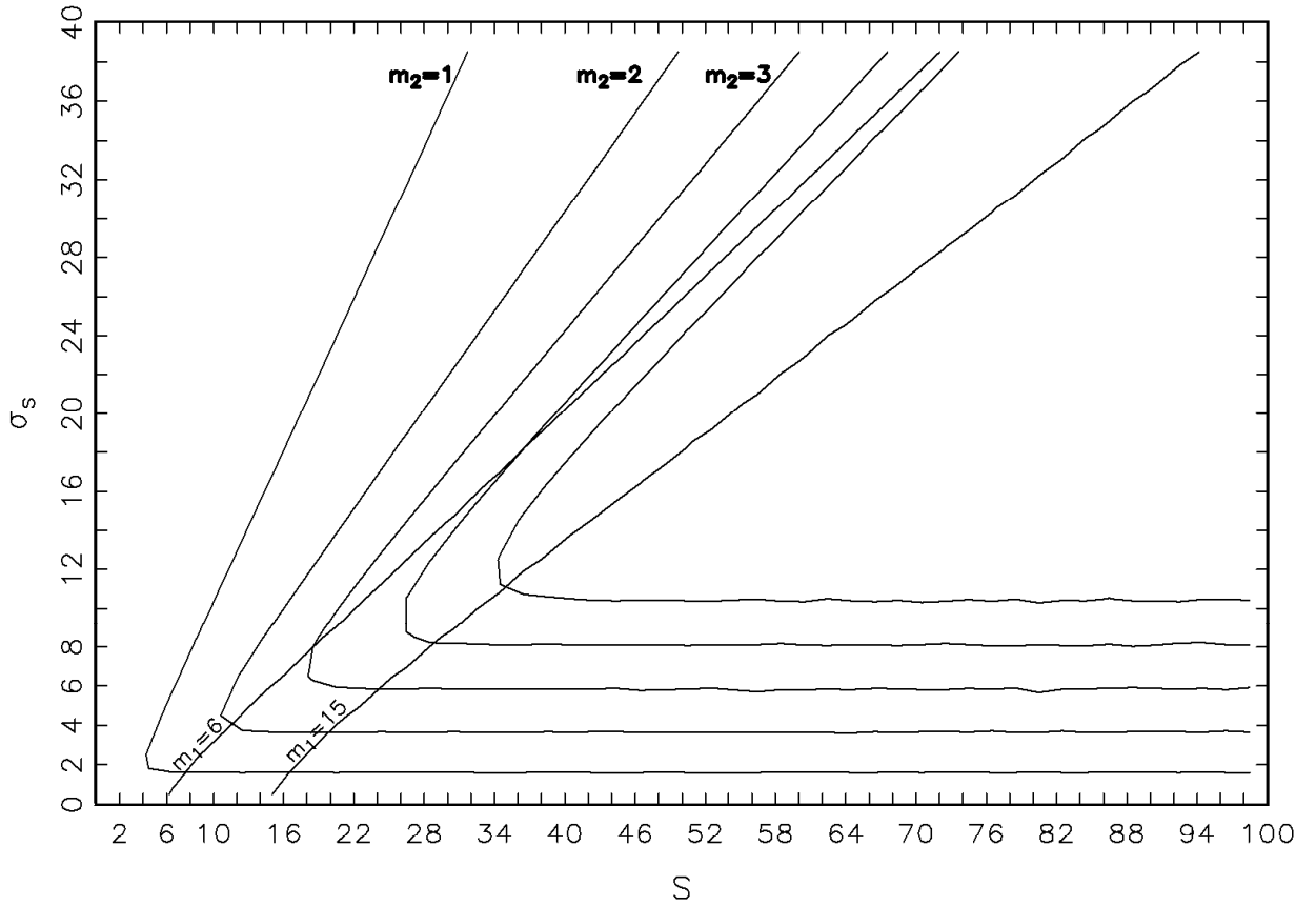
Figure E: Contour plots of mean and variance of price changes in the plane ( S , \sigma_S ) for large values of S and \sigma_S
