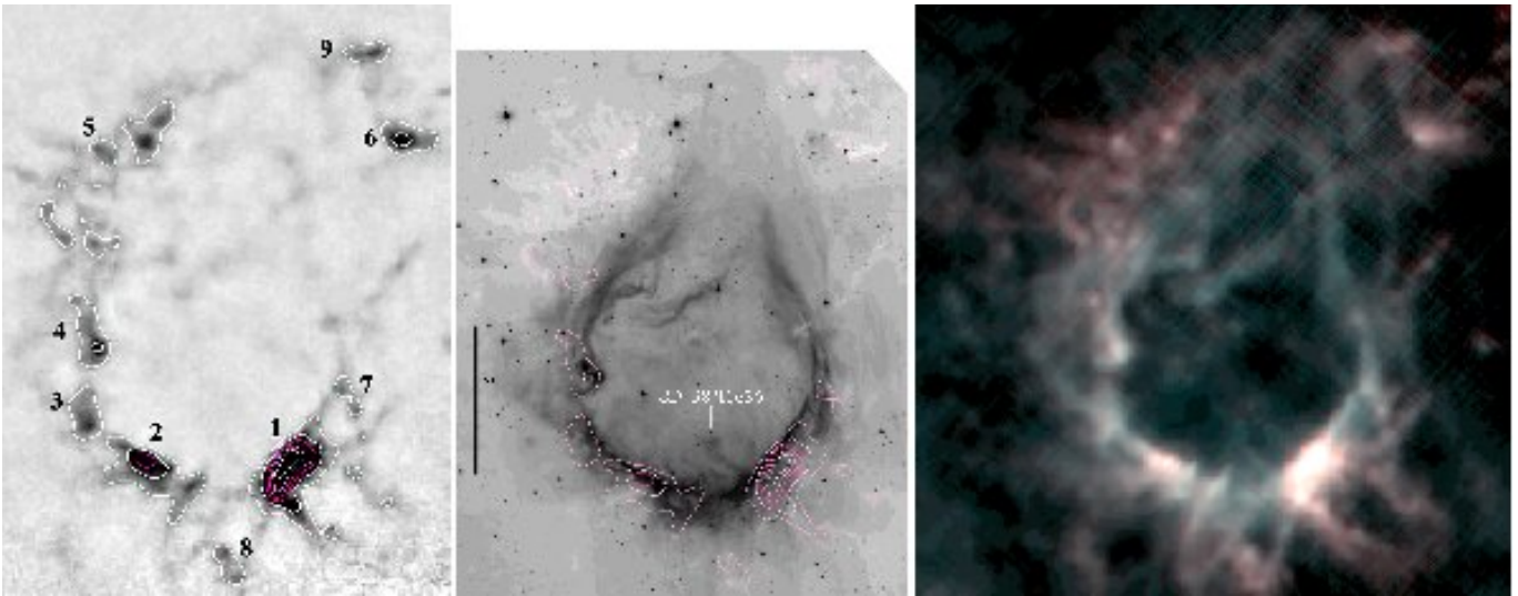
Fig. 1. A multiwavelength view of RCW 120. Left: the 870\ \mu\text{m} APEX-LABOCA image (DE09) with 870\ \mu\text{m} emission contours superimposed, as in the 8\ \mu\text{m} image. Contour levels are from 0.15 to 2.5\ \text{Jy}/\text{beam} . The condensations are identified from 1 to 9. Center: Spitzer -GLIMPSE 8\ \mu\text{m} image. The ionizing star of RCW 120, CD-38 11636, is identified. Right: Colour-composite image of RCW 120 with SPIRE 250\ \mu\text{m} (blue) and SPIRE 500\ \mu\text{m} (red). The coldest parts are clearly seen in red and match very well the position of the 870\ \mu\text{m} condensations.
