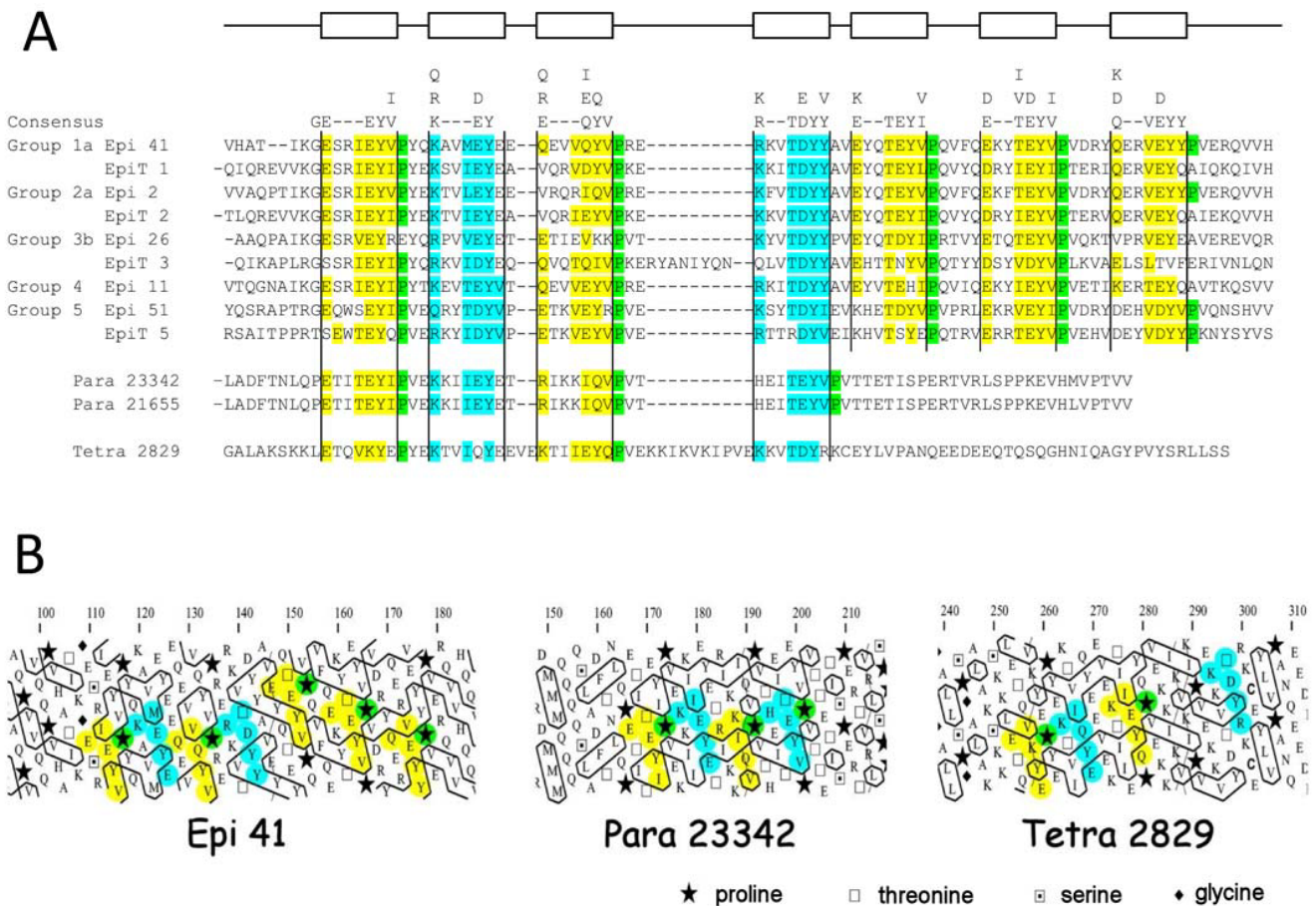
Figure 3 Modular organization of the central domain of epiplasmins. A-Alignment of the seven repeated motifs in central domains of P. tetraurelia and T. thermophila epiplasmins. Two paralogs in P. tetraurelia and one T. thermophila protein share the first half of the epiplasmin central domain. B-HCA representation of these motifs is used to consider the position of conserved amino acids in relation with the hydrophobic clusters. This shows a spatial proximity between conserved proline and tyrosine (as mentioned in the discussion).
