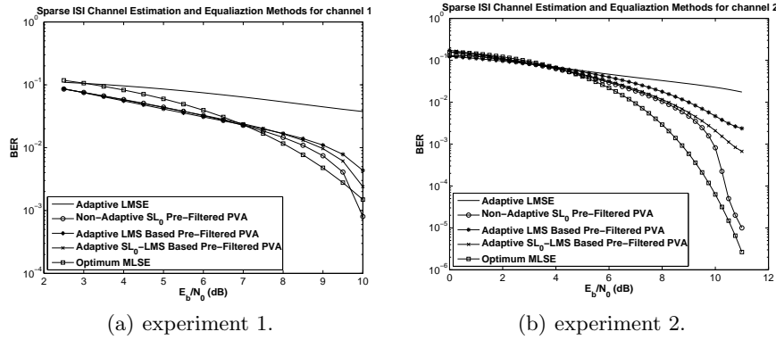
Fig. 2. Comparison of the BER-SNR curves for our estimation/equalization methods.
