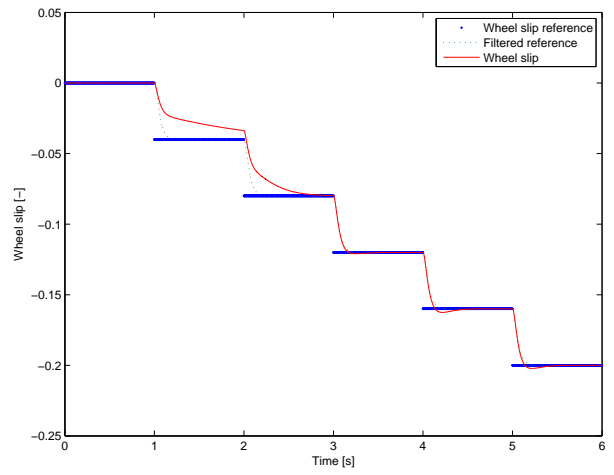
Fig. 8: Combined control with a perturbation of \mu(\cdot) .
