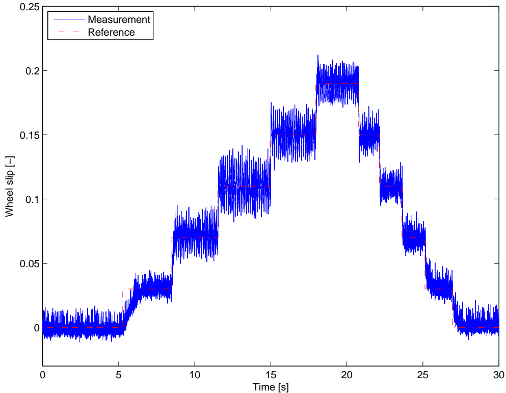
Fig. 2: Experimental validation of our our controller, when only the feedback is enabled (no feedforward).
