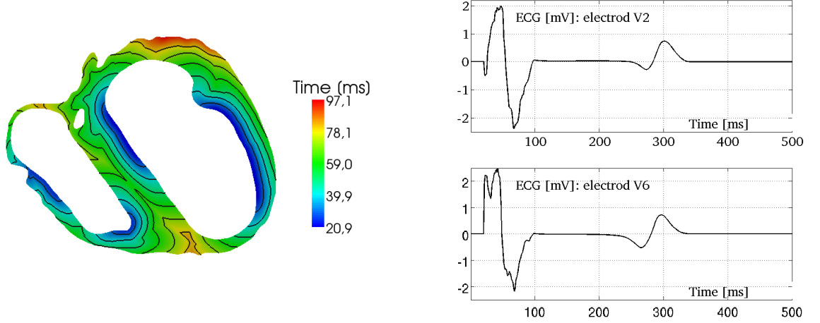
Figure 3: 2D simulation. Left: activation time in the heart, isolines in black are separated by 10 ms. Right: ECG recordings, the extra-cardiac potential is recorded on the torso surface at two points located at electrodes V2 (above) and V6 (below), see figure 1 for the electrode location.
