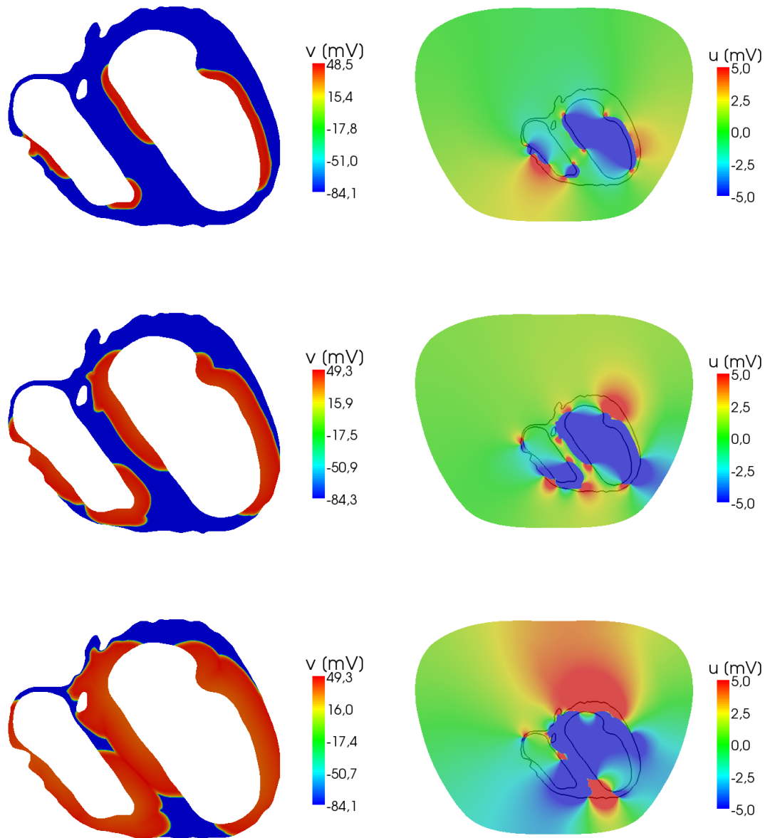
Figure 2: 2D simulation. Left: depolarisation sequence of the heart, the transmembrane potential v is represented 15, 30 and 45 ms after stimulation. Right: associated potential u in the heart and in the extra cardiac region.
