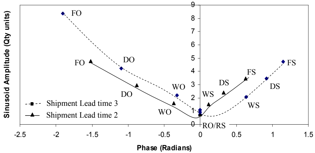
a) Simulated Beer Game with Parameters T_i 3, T_a 1.5, T_w 3
