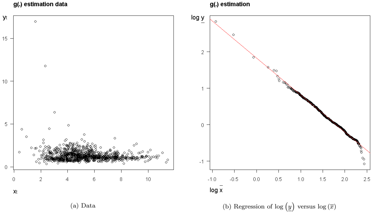
Figure 2.1: g estimation
