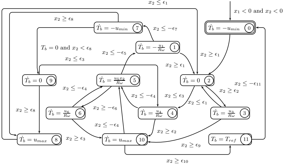
Figure 5: Our eleven-phase ABS regulation logics. The first five phases coincide with those of Figure 2.
