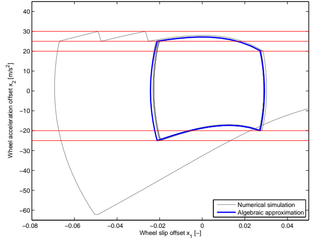
Figure 4: Limit cycle obtained for \epsilon_1 = \epsilon_5 = 20 and \epsilon_3 = \epsilon_4 = 25 , in the case u_5 = 200 , also with \epsilon_2 = 33 but with u_3 = 10^5 (obtained with the formulas of [1]).
