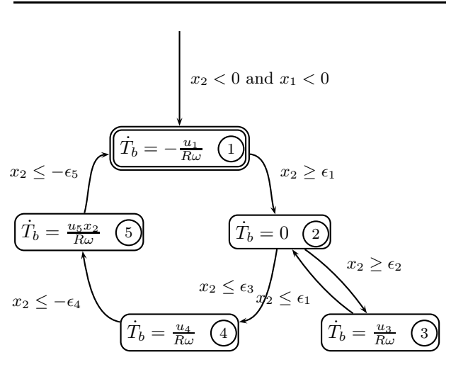
Figure 2: The five-phase ABS regulation logic.
