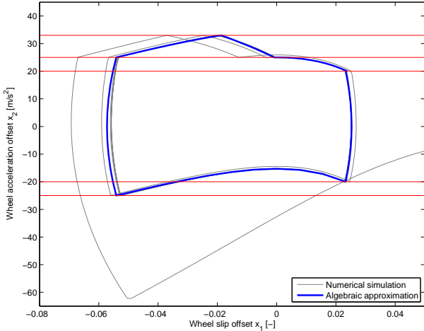
Figure 3: Limit cycle obtained for \epsilon_1 = \epsilon_5 = 20 and \epsilon_3 = \epsilon_4 = 25 , in the case u_5 = 0 , with \epsilon_2 = 33 and u_3 = 12970 (obtained with the formulas of [6]).
