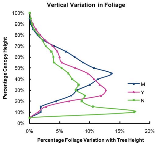
Figure 3. Variation of canopy foliage with tree height in the three poplar stands.
