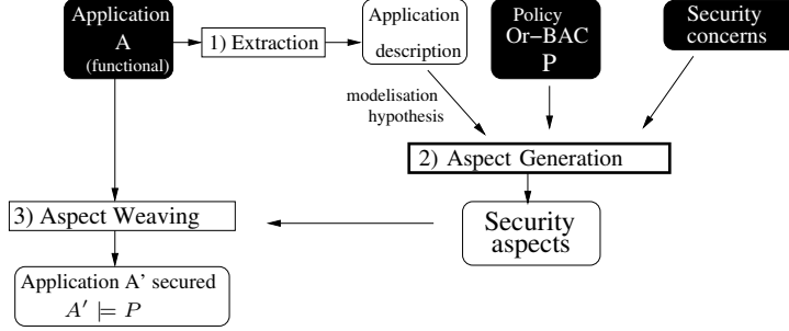
Fig. 1: Approach overview.
