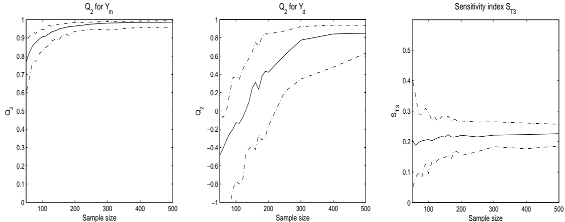
Fig. 2 For the Ishigami function and the joint Gp model, median and 90%-confidence interval of Q_2(Y_m) (left), Q_2(Y_d) (center) and estimated S_{T_3} in function of the learning sample size n .
