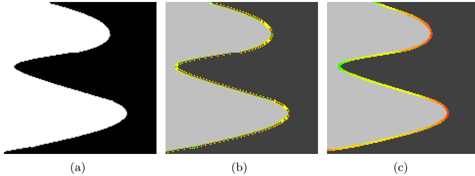
FIGURE 11. The curvature color display rule. Zero curvatures are displayed in yellow, positive curvatures are shown in a gradation from yellow to red, and negatives from yellow to green. The initial image (a) had its curvatures computed in two different ways: by an FDS by formula (1) (b), and by LLS (c). In the first case the curvature presents oscillations, whereas the second result is coherent with our perception.
