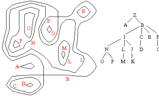
FIGURE 3. Tree of bilinear level lines.
