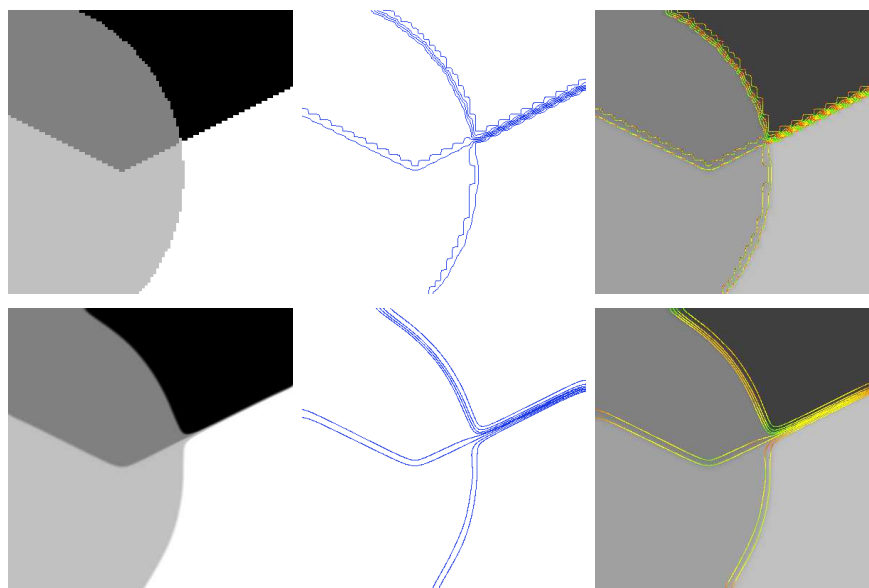
FIGURE 18. Top: original image, extracted level lines, non-filtered curvatures. Bottom: LLAS image, smoothed level lines and curvature map.
