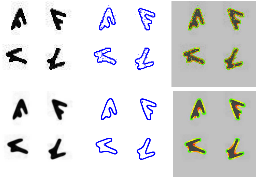
FIGURE 22. Top: original image, its corresponding level lines and curvatures. Bottom: LLAS evolution, affine smoothed level lines and curvature map after filtering.
