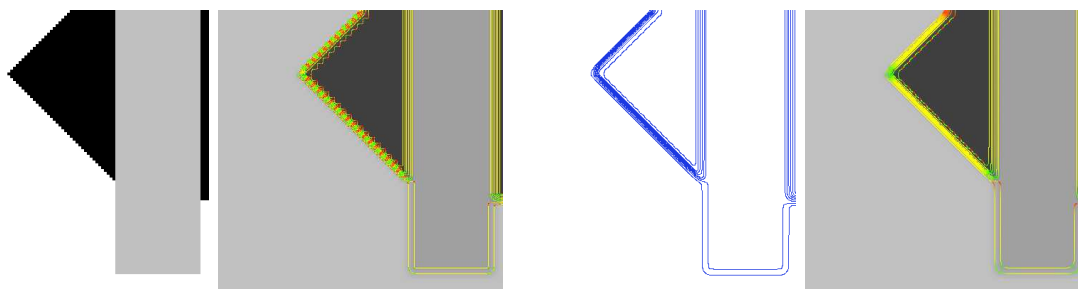
FIGURE 17. Original image, non-filtered curvatures, smoothed level lines by LLAS and curvature map.
