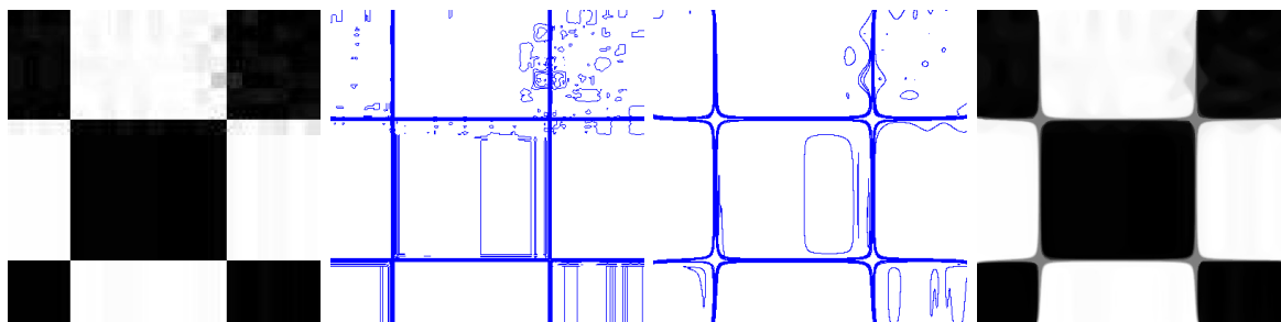
FIGURE 4. Fattening effect. From left to right, the original image, its extracted level lines with quantization step s = 16 , their independent evolution by affine shortening at renormalized scale l = 8 and the image reconstructed from the evolved level lines. Observe that distinct, touching level lines tear apart and non-empty interiors appear at the saddle points. At these points four squares, two black, two white, meet initially by their corners. After evolution, fattened grey regions are liberated by the retraction of the square level lines surrounding the black and the white squares.
