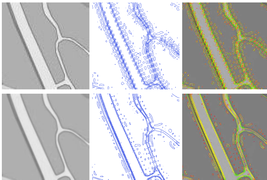
FIGURE 25. Top: Piece of map with roads, its corresponding level lines and curvatures. Bottom: LLAS evolution, affine smoothed level lines and curvature map after filtering.
