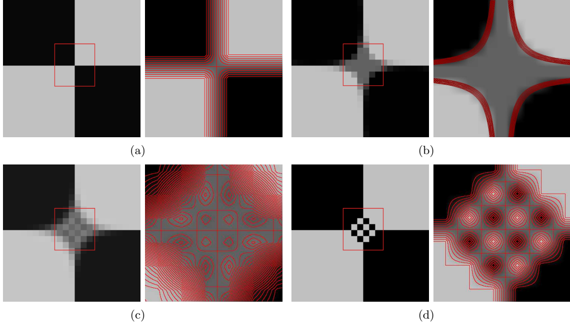
FIGURE 6. The four pairs present various implementations of the mean curvature motion on a checkerboard image (left column) and zooms at an X-junction, with its level lines overprinted on the image (right). From top to bottom : (a). original image (the zoom is by bilinear interpolation), (b). Level lines shortening, (c). Finite difference scheme, (d) FDS stack filter. Only LLS does not create new extrema.
