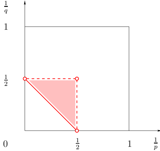
FIGURE 2. Admissibility in dimension n = 3
