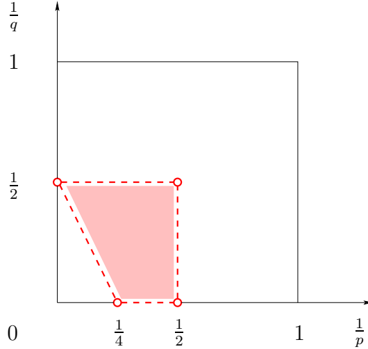
FIGURE 4. Admissibility in dimension n=2
