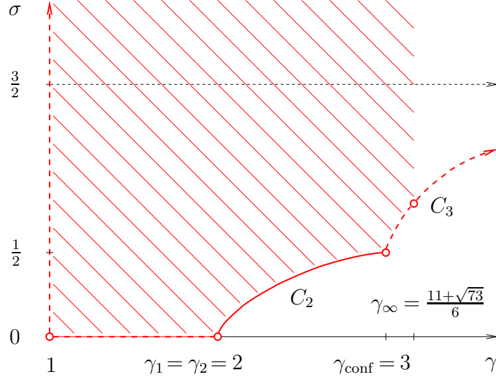
FIGURE 6. Regularity in dimension n=3
