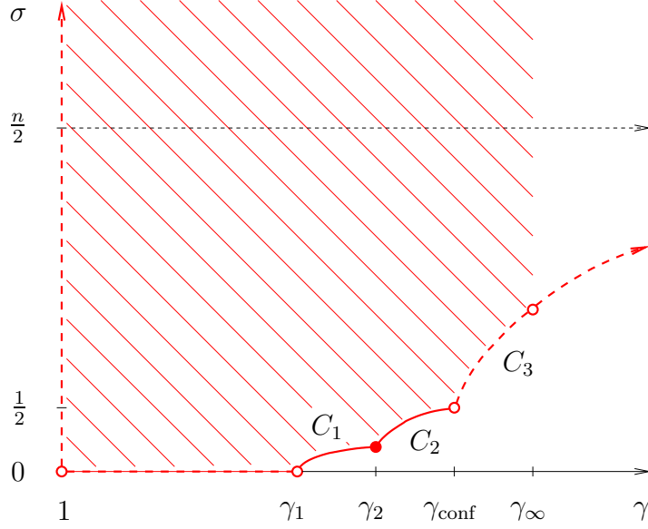
FIGURE 5. Regularity in dimension n \geq 4
