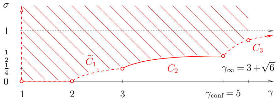
FIGURE 7. Regularity in dimension n=2
