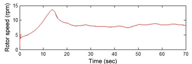
Fig. 13. Rotor speed.
