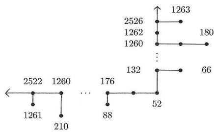
Figure 7: T_N(f''_0)
