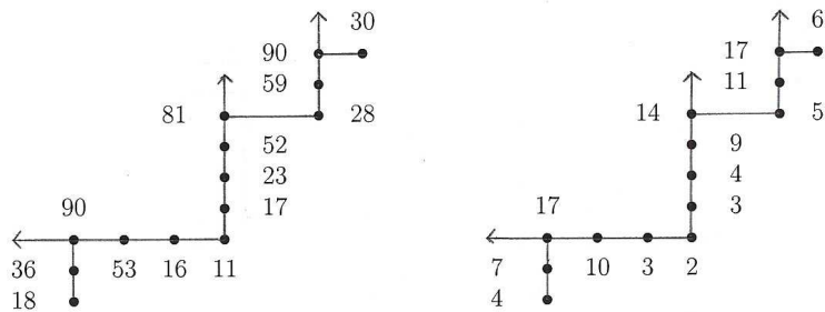
Figure 10: T_N(g_0) T_\nu(g_0)
