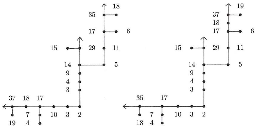
Figure 13: T_\nu(g_0')
