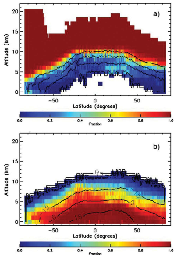
FIG. 9. Zonal mean fraction of ice cloud and water cloud for Aug 2007. (a) contours = -30^{\circ} , -20^{\circ} , -10^{\circ} , 0^{\circ} C; (b) contours = -30^{\circ} , -15^{\circ} , 0^{\circ} , +15^{\circ} C.
