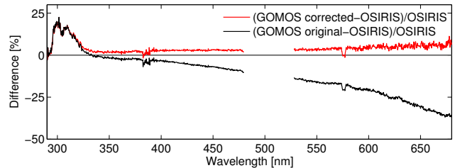
Fig. 7. Example of radiance ratios from GOMOS and OSIRIS. Upper panel: ratios of 30 and 47 km. Lower panel: relative differences.
