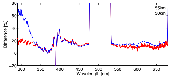
Fig. 6. Median relative difference of the 14 OSIRIS and stray light corrected GOMOS absolute radiances at 30 km (blue) and 55 km (red).
