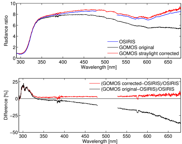
Fig. 7. Example of radiance ratios from GOMOS and OSIRIS. Upper panel: ratios of 30 and 47 km. Lower panel: relative differences.
