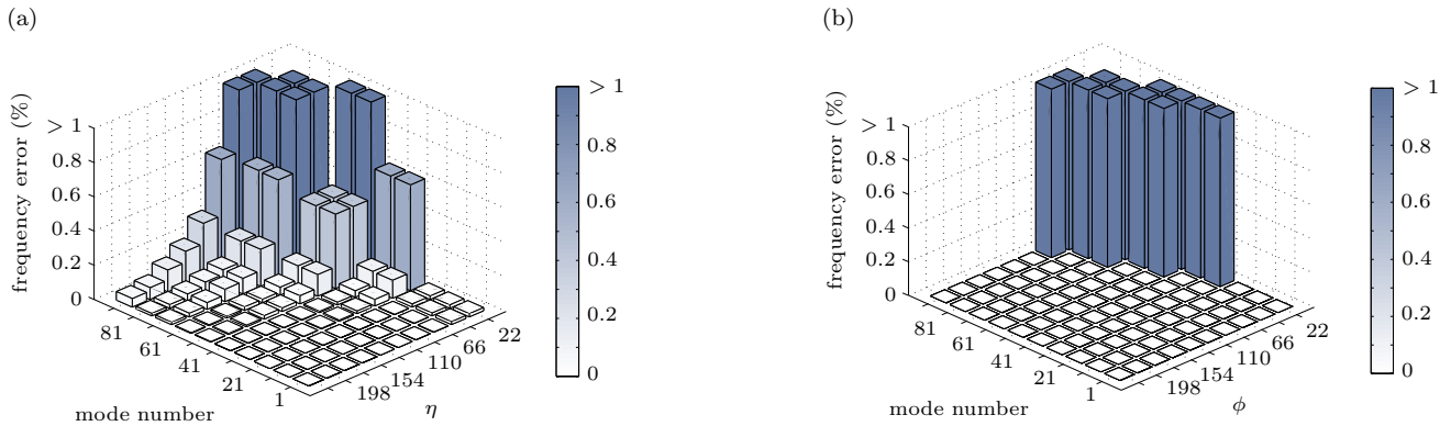
Figure 10: Convergence of the reduced order models obtained with each component mode synthesis method toward the finite element model: (a) CB reduced order model; (b) CM reduced order model.
