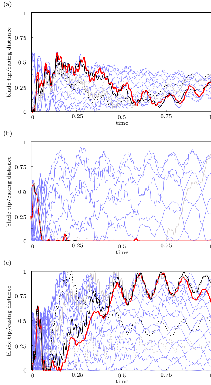
Figure 12: Convergence of the results obtained with CB method \eta = 0 (---); \eta = 44 (-.-.-); \eta = 88 (—); \eta = 220 (—); u_{fe}(t) (—). (a) damped motion, blade 10, \Omega = 0.56 , k = 2 ; (b) locked motion, blade 9, \Omega = 1.12 , k = 2 ; (c) sustained motion, blade 2, \Omega = 1.28 , k = 3 .
