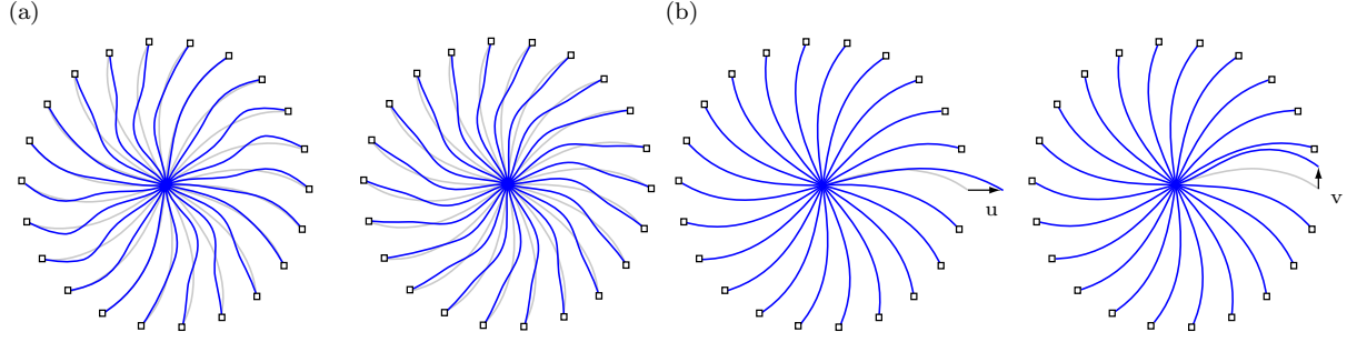
Figure 6: Craig-Bampton method: (a) component modes; (b) constrained modes.
